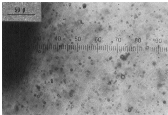
FIGURE 1 Micrograph of the emulsion formed in a 5% methanol + water solution of the surface-active dye at 7.99 \times 10^{-3} M.
